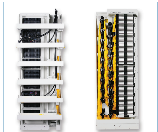
Centrix Frame | Photos CRR2014; CRR3616
